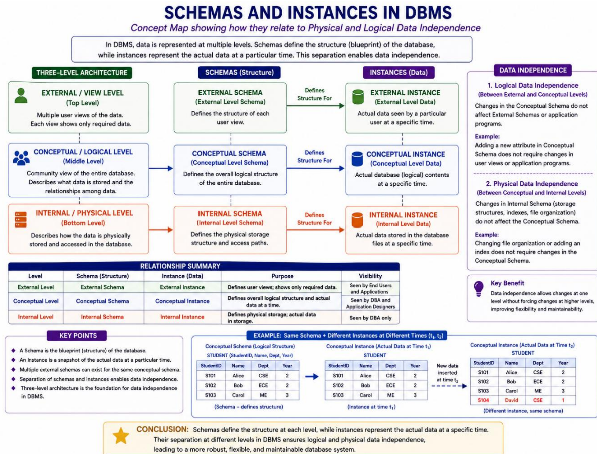
Figure 9: Concept Map of Schema, Instance, and Data Independence
