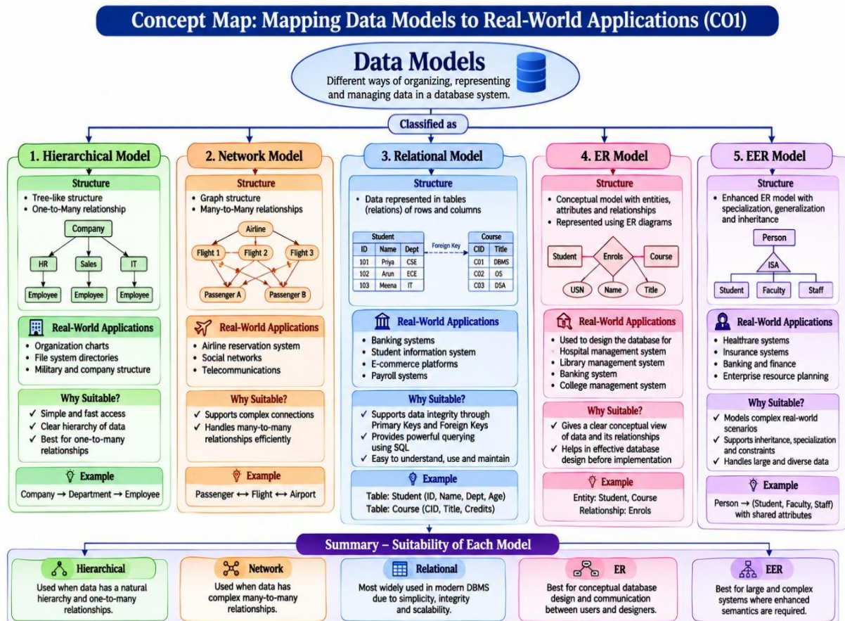
Figure 8: Concept Map of Data Models and Their Real-World Applications
