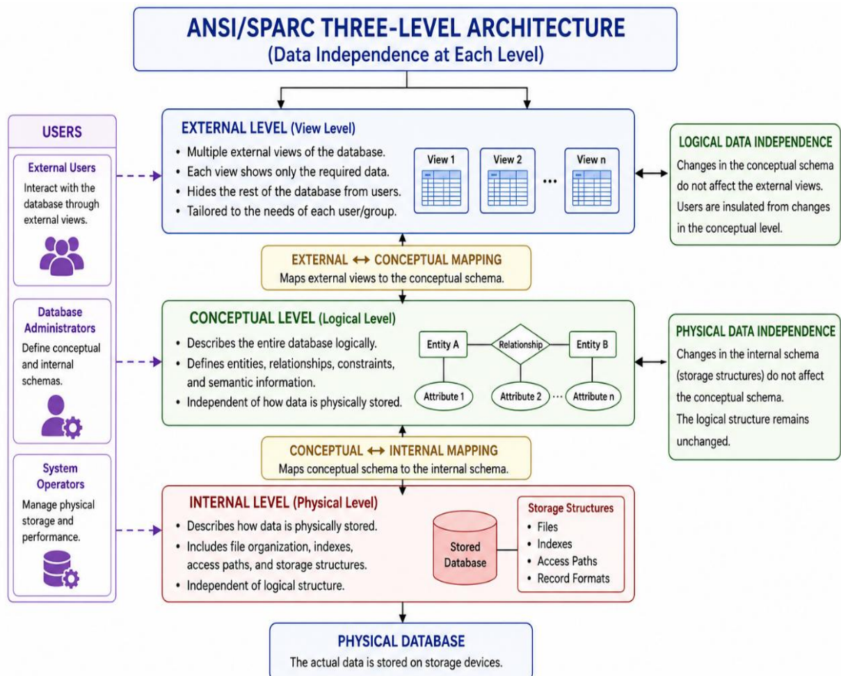
Figure 2: Concept Map of the Three-Level ANSI/SPARC Architecture and Data Independence
