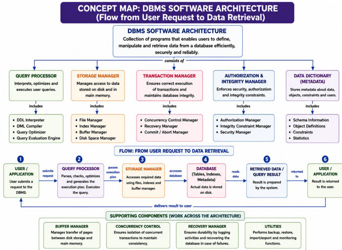
Figure 7: Concept Map of DBMS Software Architecture
