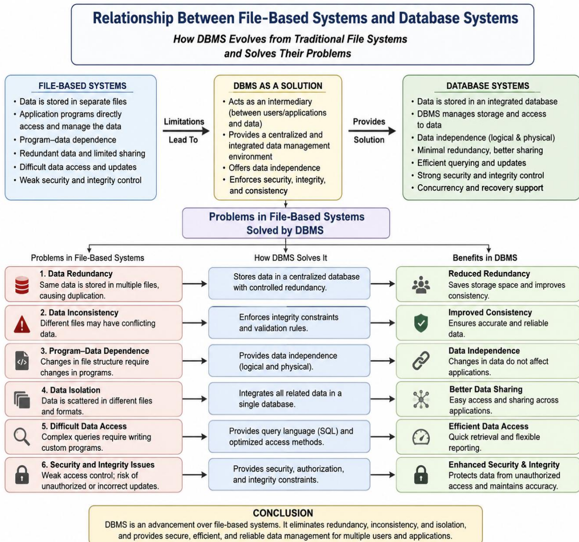
Figure 3: Concept Map Comparing File-Based Systems and Database Management Systems
